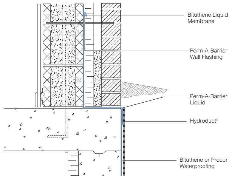
Perm-A-Barrier Liquid Foundation Wall Detail
