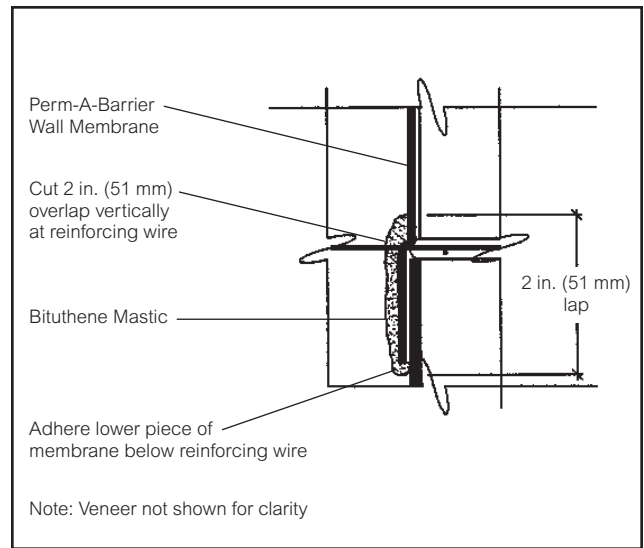
Figure 2: Horizontal Reinforcing
