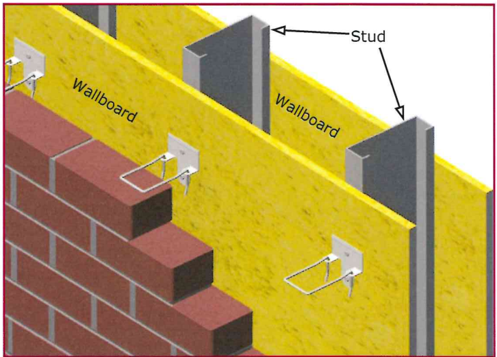
Tying Masonry To Steel Stud
