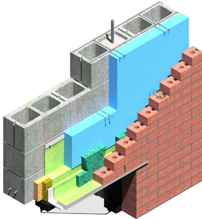
ISOMETRIC VIEW
