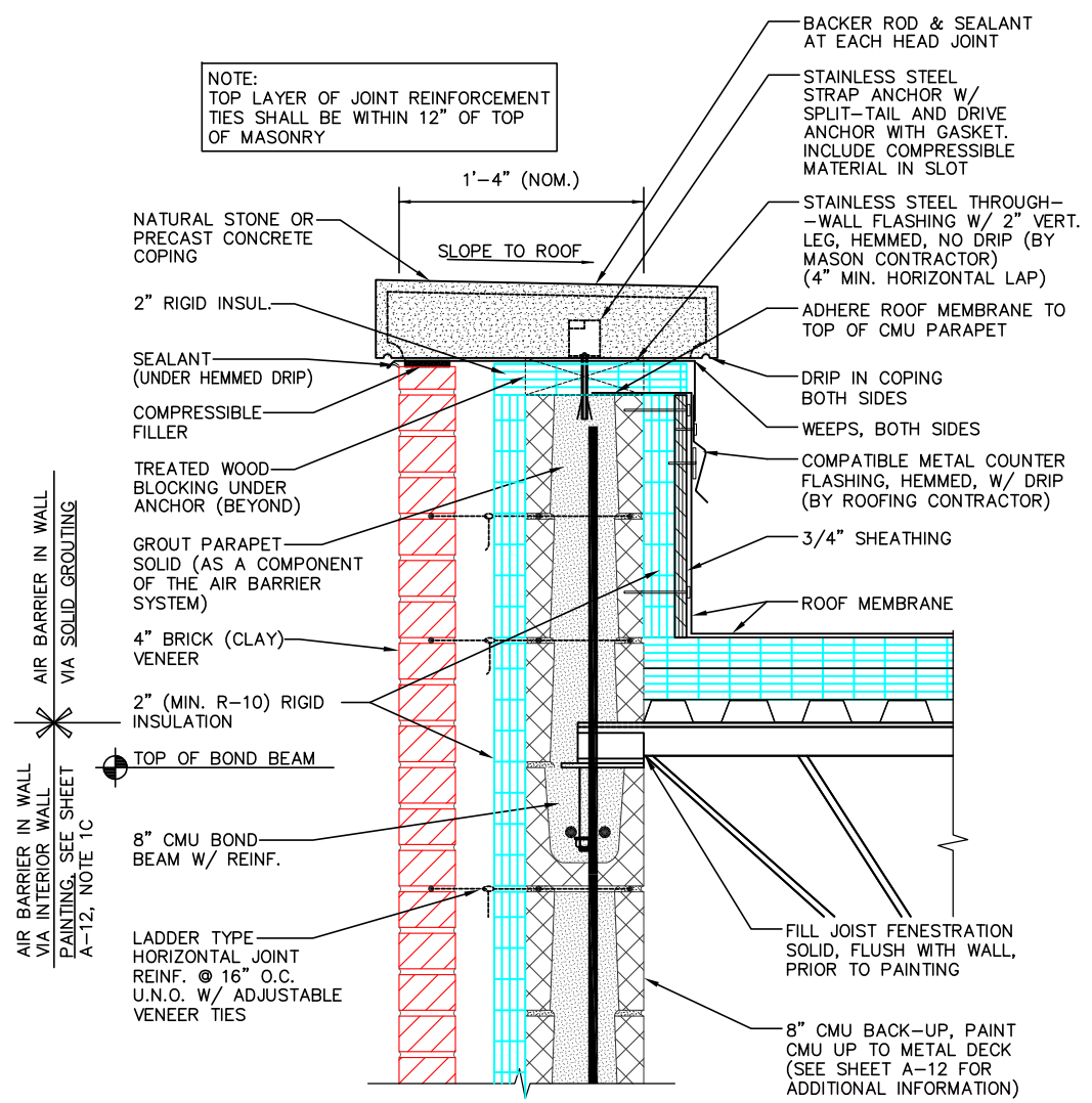
SECTION VIEW
