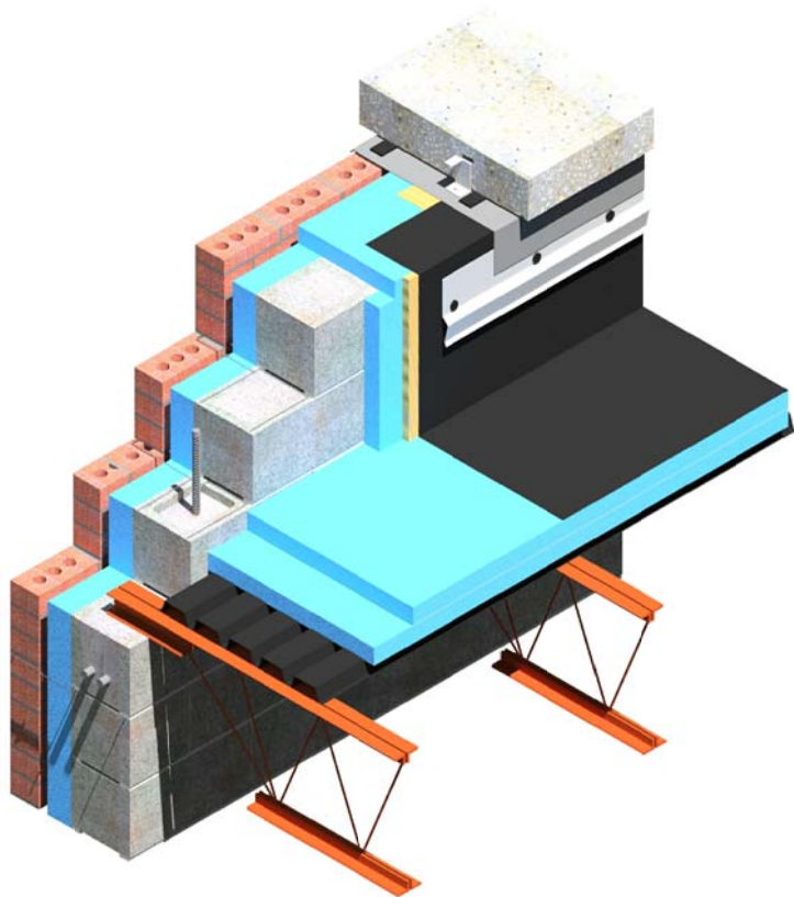
ISOMETRIC VIEW
