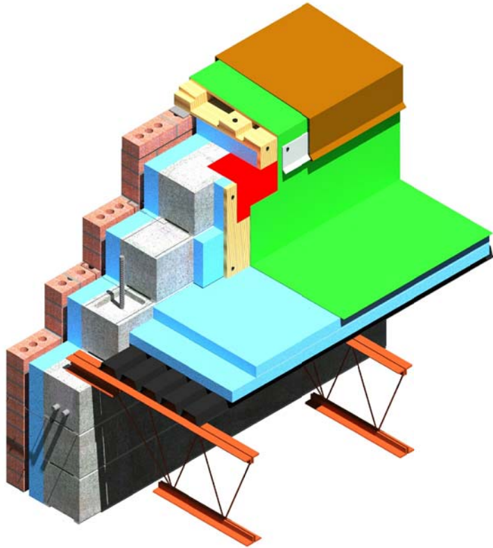
ISOMETRIC VIEW
