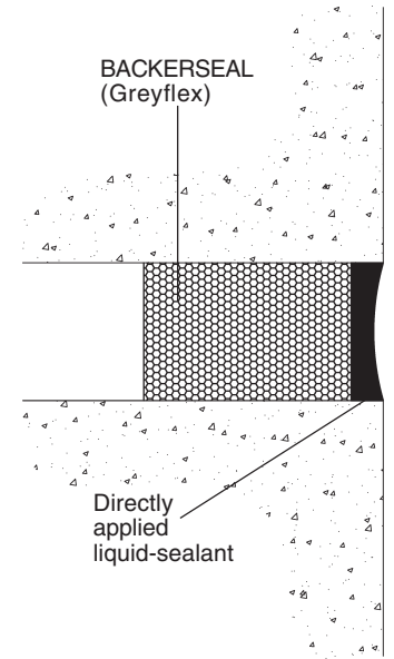
BACKERSEAL (Greyflex) as part of a hybrid sealant system with directly-applied liquid sealant.
