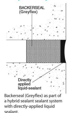
Figure 2: As part of a binary sealant system
