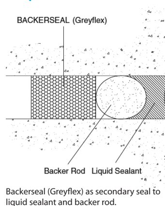
Figure 1: As a secondary sealant to liquid sealant with backer-rod.
