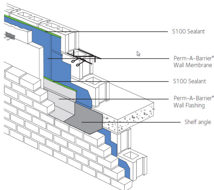
Typical Air and Vapor Barrier Application
